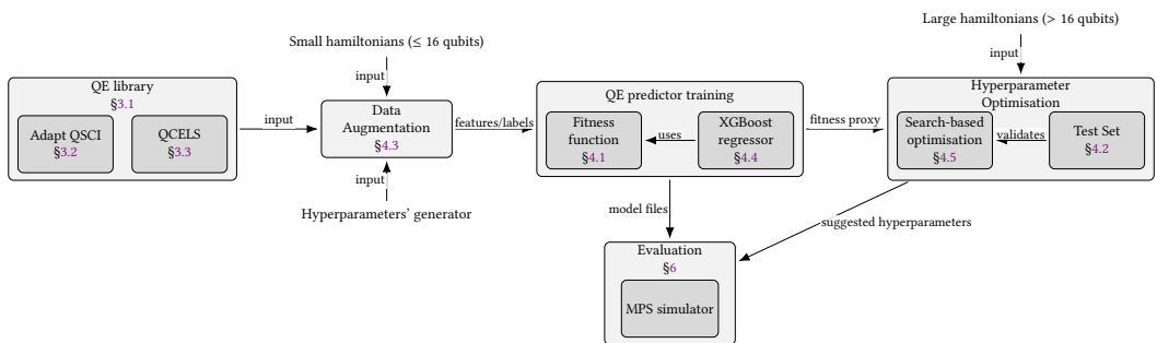
Fig. 1. AccelerQ at a glance: inputs from the QE library feed data augmentation and training ( QE predictor ), which serves as a fitness proxy for hyperparameter optimisation; suggestions are evaluated on a simulator.
