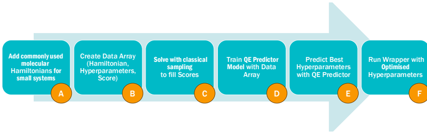
Fig. 5. AccelerQ process: Classical pre-processing, QE predictor model training on smaller systems and generalisation on bigger systems
