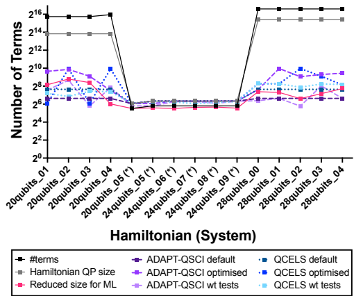
Fig. 8. Number of Hamiltonian terms (Y-axis, \log_2 scale) for QE predictor queries and QE implementation executions across different systems (X-axis), shown as raw and compressed sizes.
